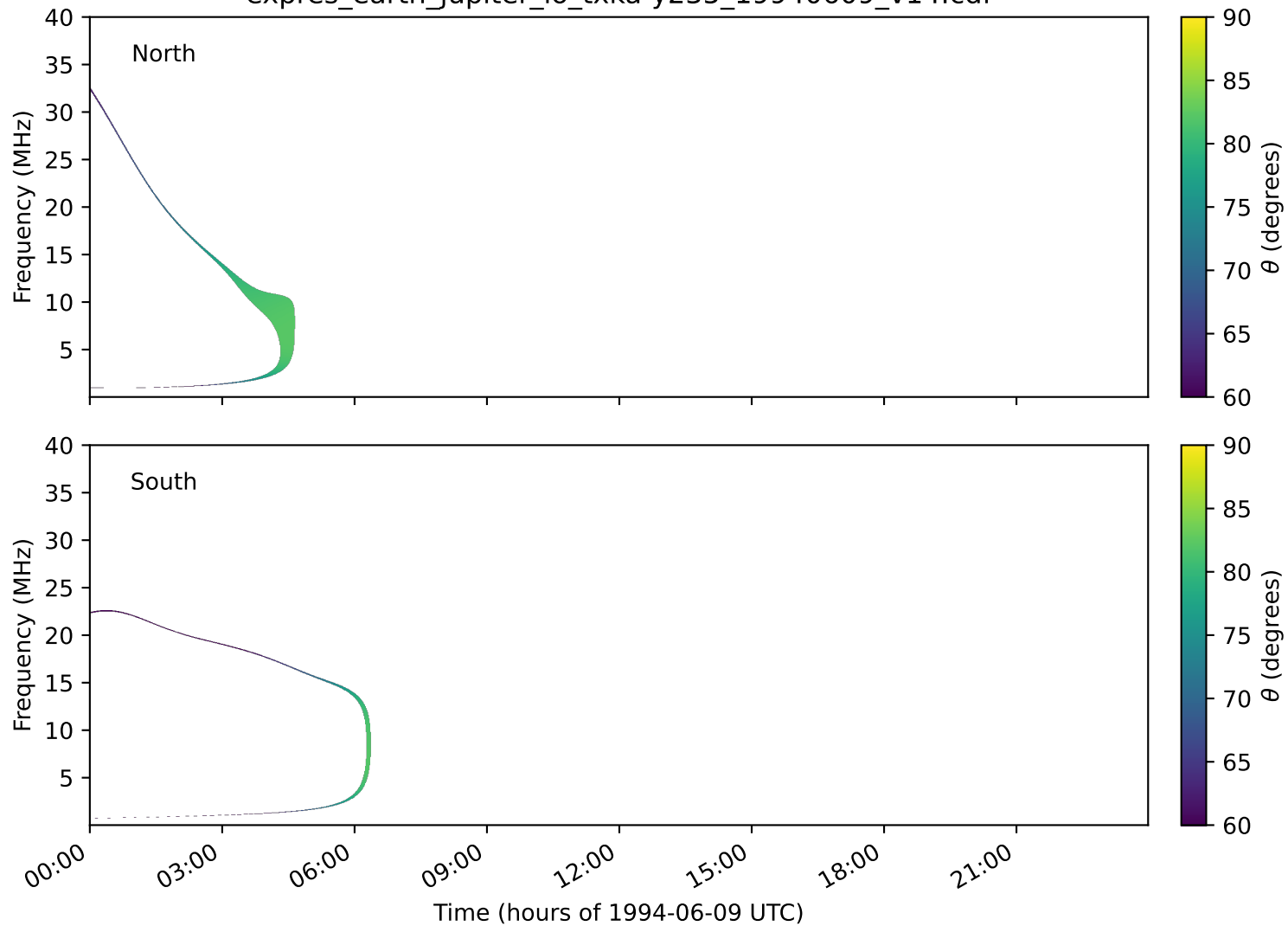
expres_earth_jupiter_io_txka-y235_19940609_v14.cdf
