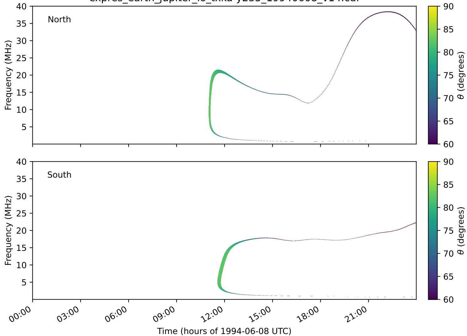
expres_earth_jupiter_io_txka-y235_19940608_v14.cdf
