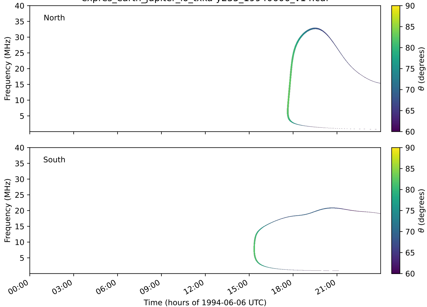
expres_earth_jupiter_io_txka-y235_19940606_v14.cdf
