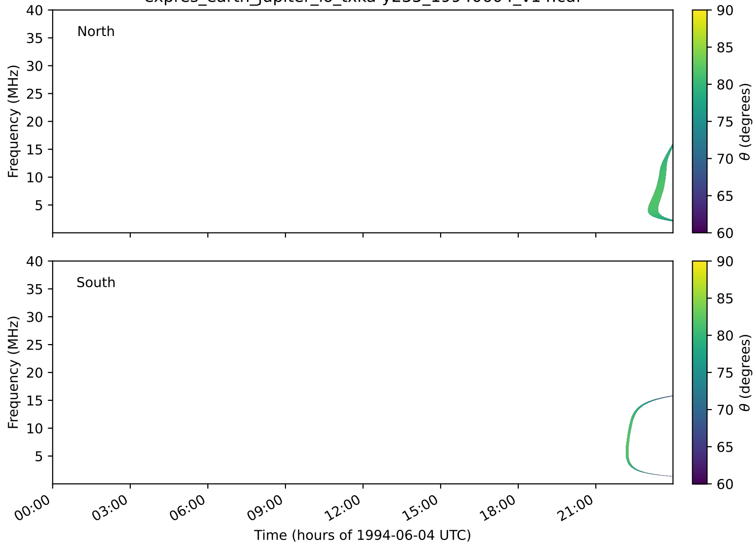
expres_earth_jupiter_io_txka-y235_19940604_v14.cdf
