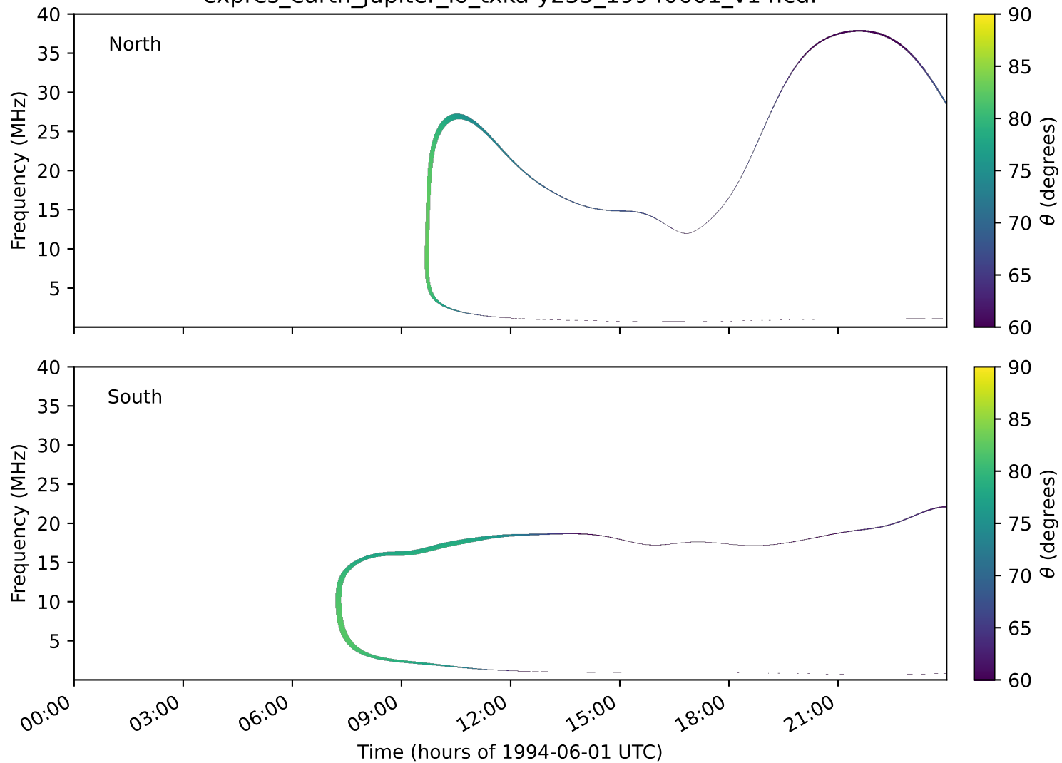
expres_earth_jupiter_io_txka-y235_19940601_v14.cdf
