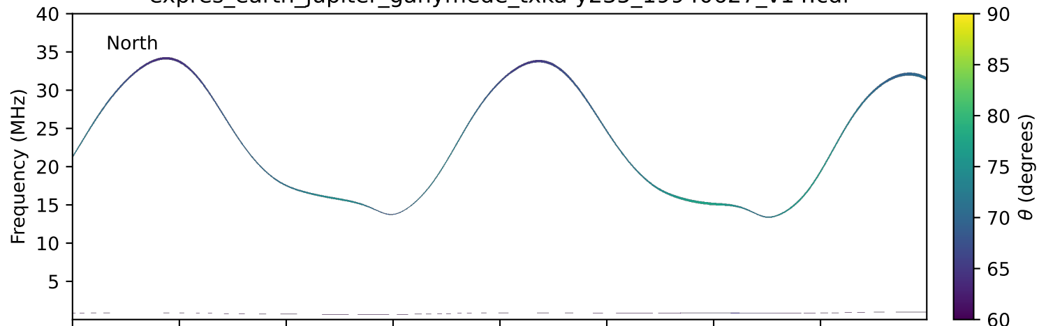
expres_earth_jupiter_ganymede_txka-y235_19940627_v14.cdf
