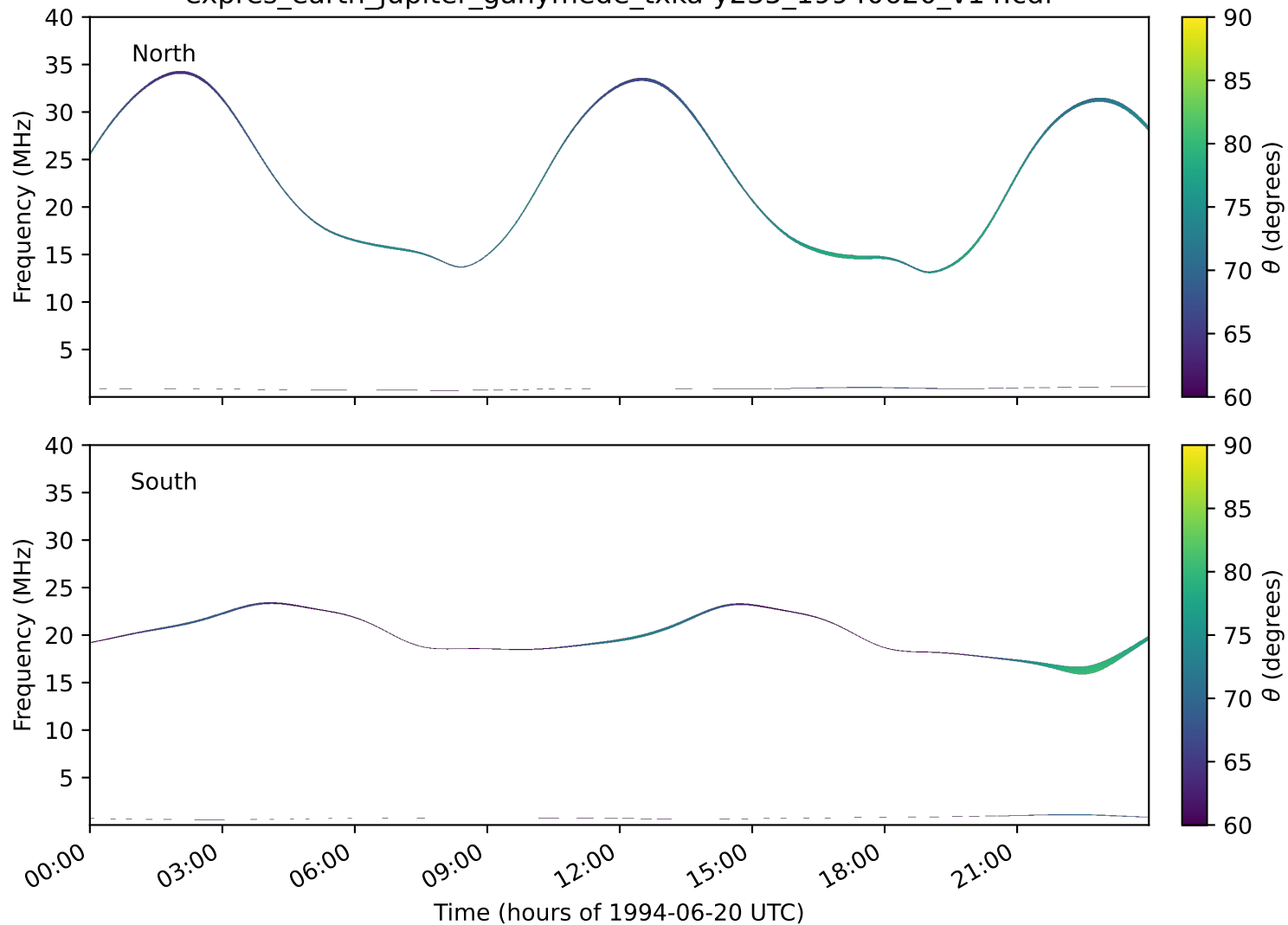
expres_earth_jupiter_ganymede_txka-y235_19940620_v14.cdf
