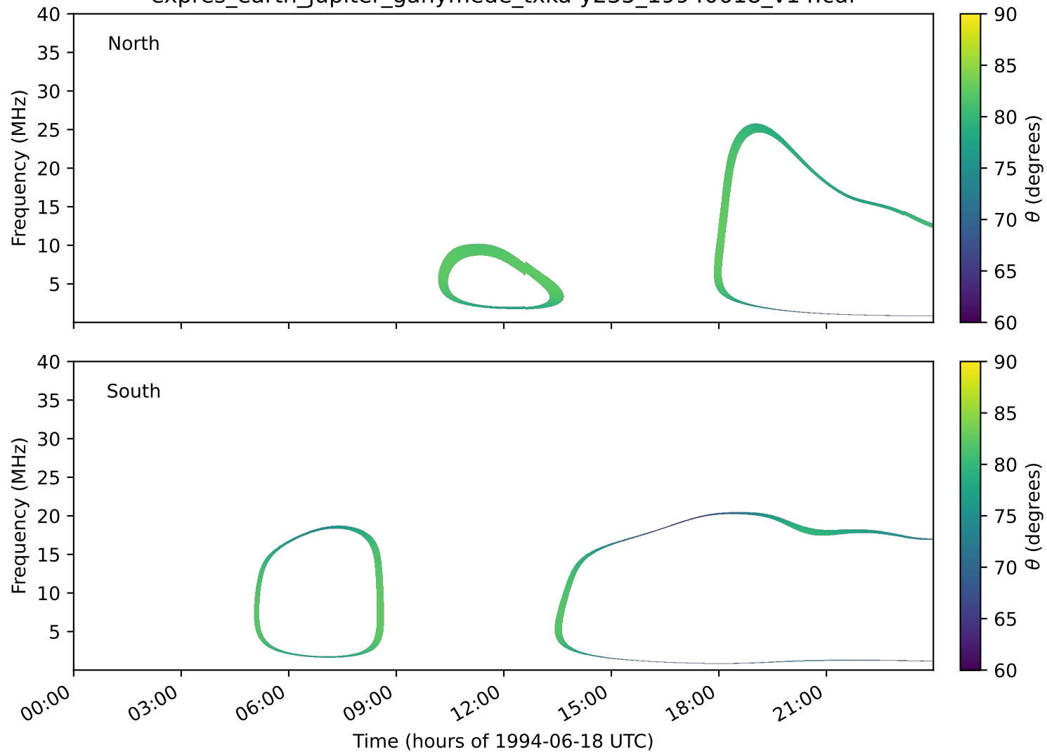
expres_earth_jupiter_ganymede_txka-y235_19940618_v14.cdf
