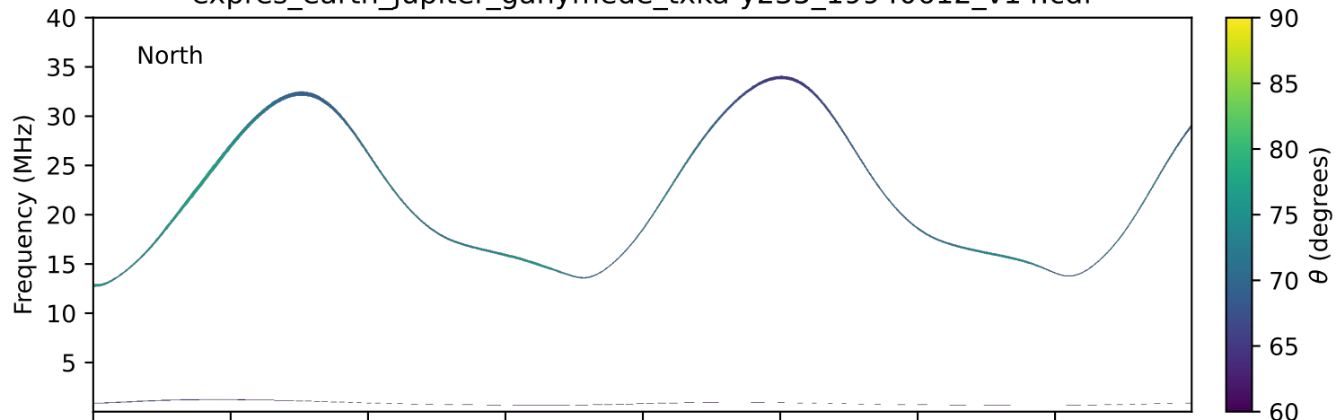
expres_earth_jupiter_ganymede_txka-y235_19940612_v14.cdf
