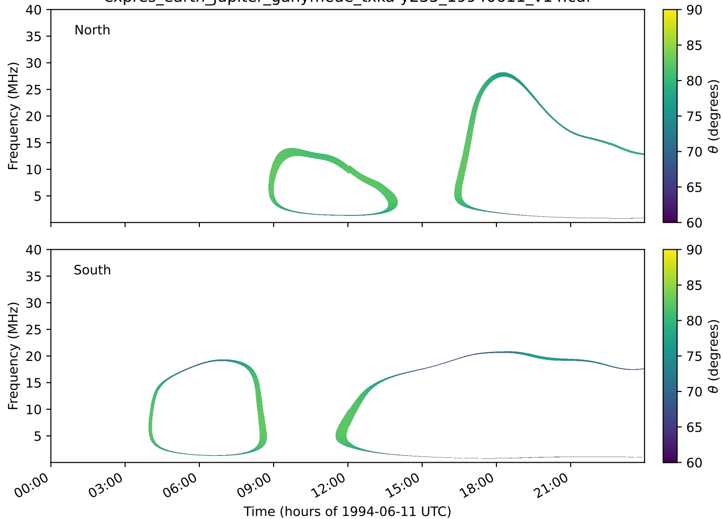
expres_earth_jupiter_ganymede_txka-y235_19940611_v14.cdf
