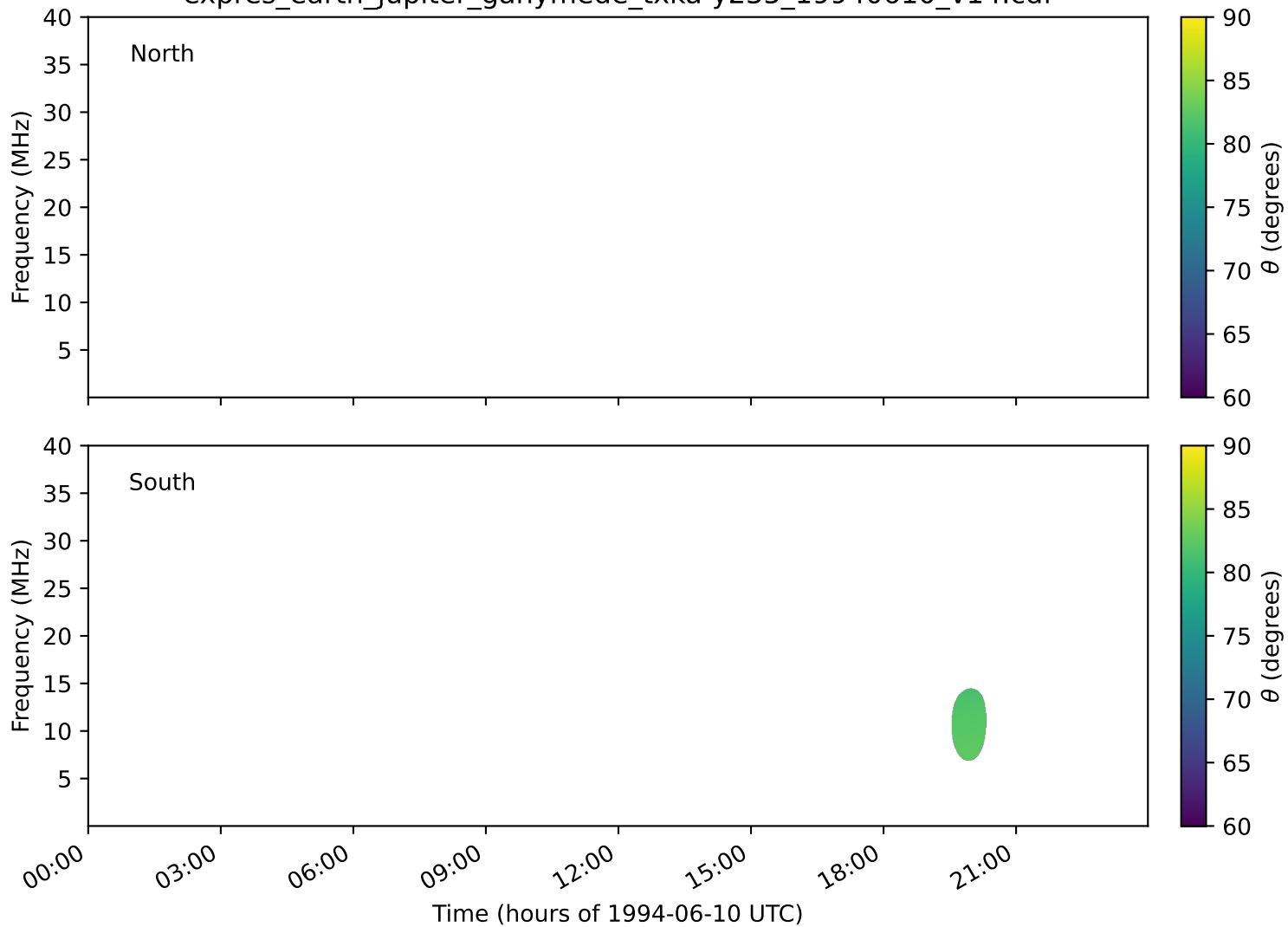
expres_earth_jupiter_ganymede_txka-y235_19940610_v14.cdf
