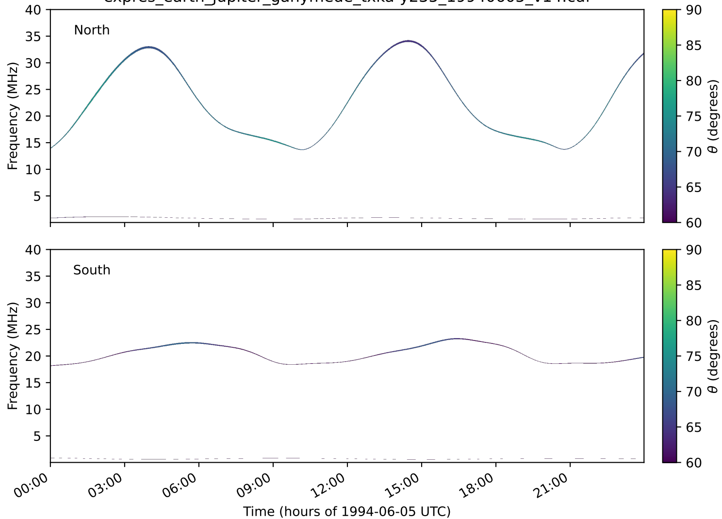
expres_earth_jupiter_ganymede_txka-y235_19940605_v14.cdf
