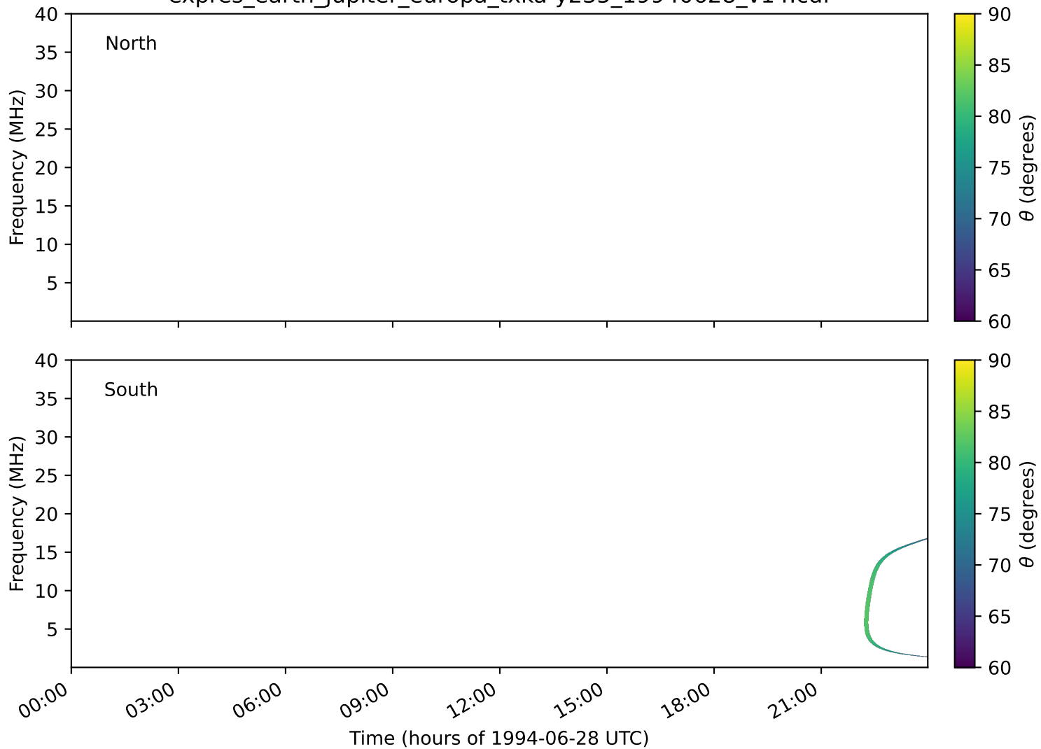
expres_earth_jupiter_europa_txka-y235_19940628_v14.cdf
