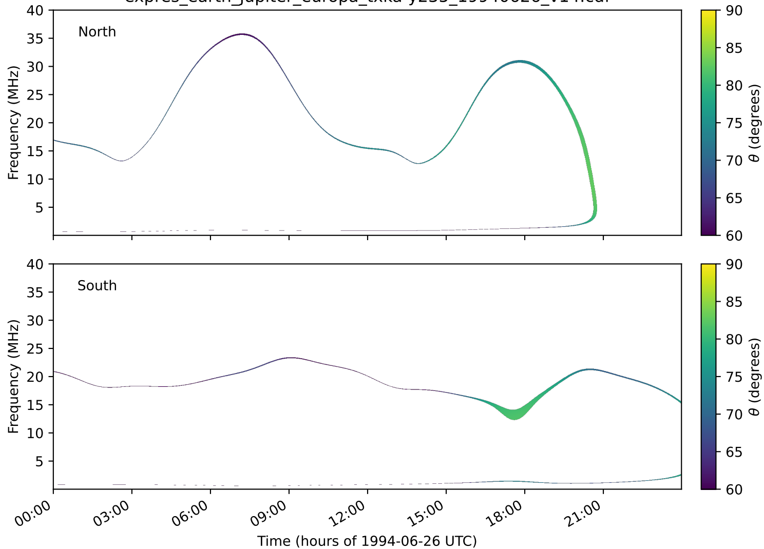
expres_earth_jupiter_europa_txka-y235_19940626_v14.cdf
