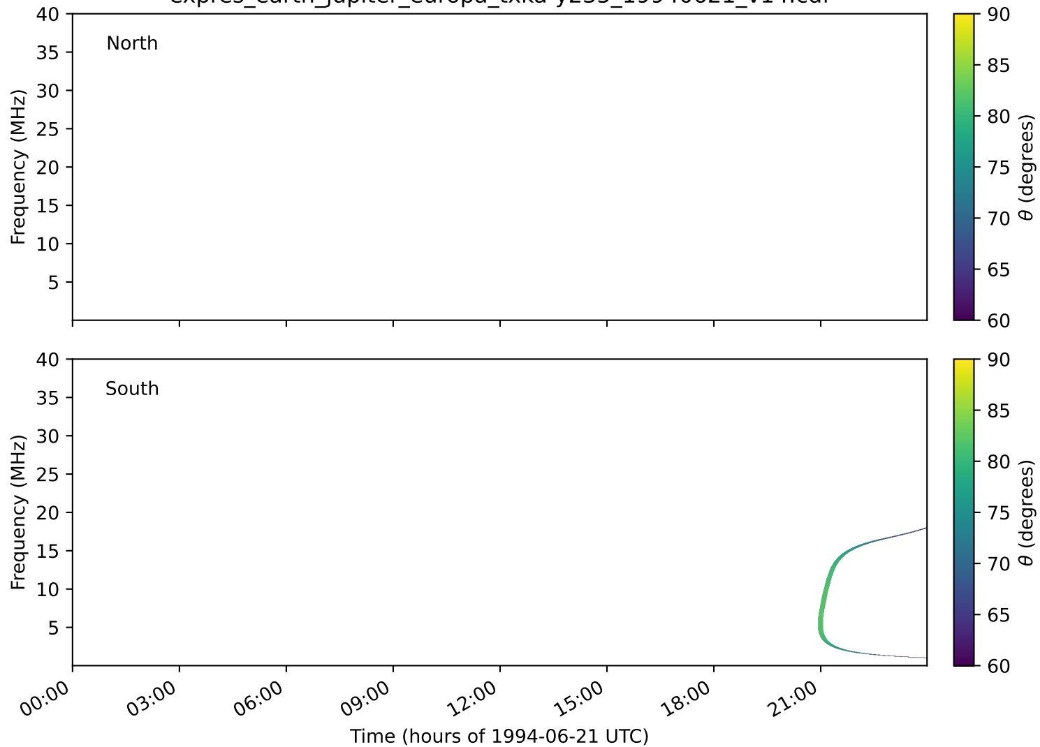
expres_earth_jupiter_europa_txka-y235_19940621_v14.cdf
