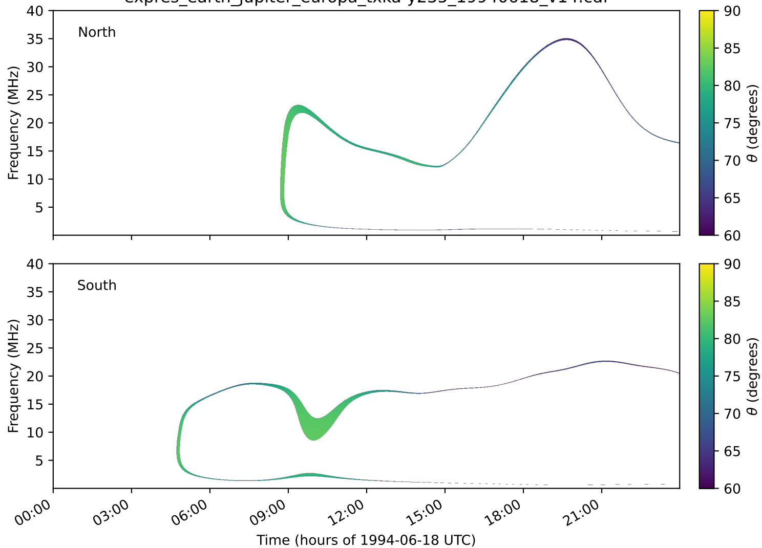
expres_earth_jupiter_europa_txka-y235_19940618_v14.cdf
