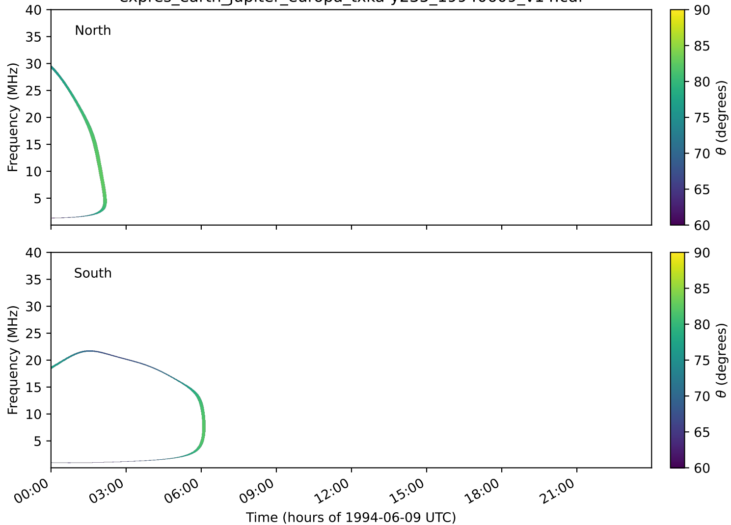
expres_earth_jupiter_europa_txka-y235_19940609_v14.cdf
