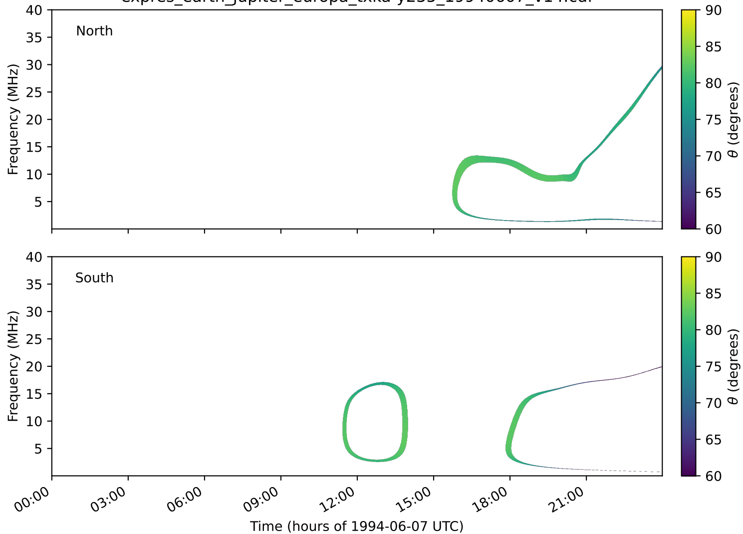
expres_earth_jupiter_europa_txka-y235_19940607_v14.cdf
