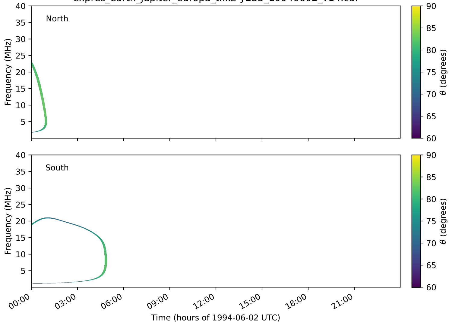
expres_earth_jupiter_europa_txka-y235_19940602_v14.cdf
