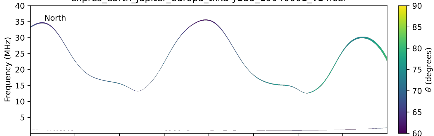
expres_earth_jupiter_europa_txka-y235_19940601_v14.cdf
