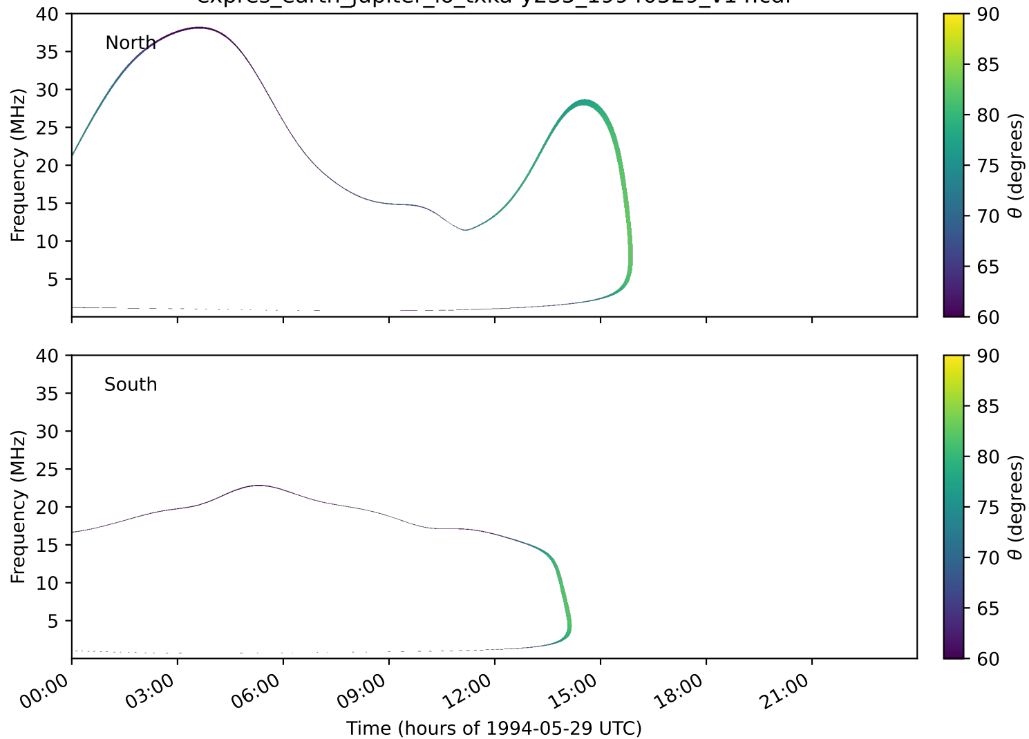
expres_earth_jupiter_io_txka-y235_19940529_v14.cdf
