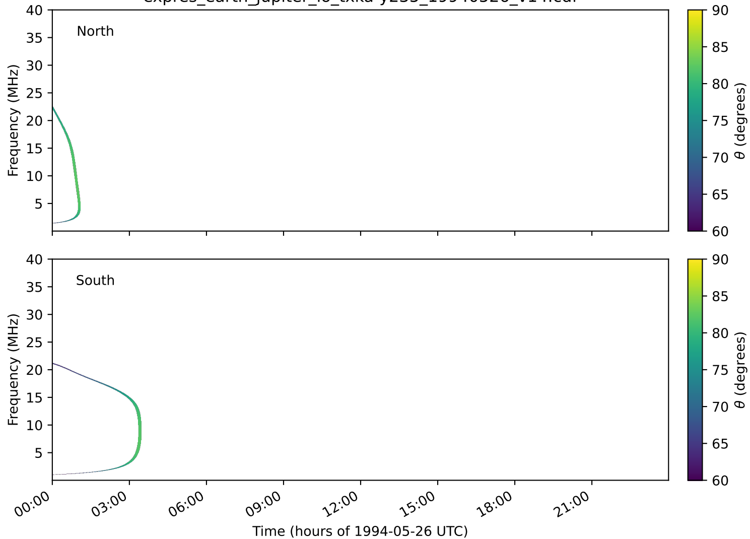
expres_earth_jupiter_io_txka-y235_19940526_v14.cdf
