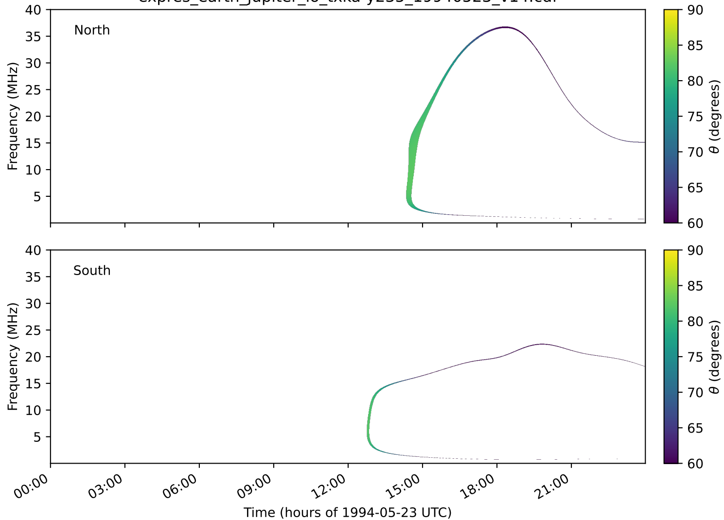
expres_earth_jupiter_io_txka-y235_19940523_v14.cdf
