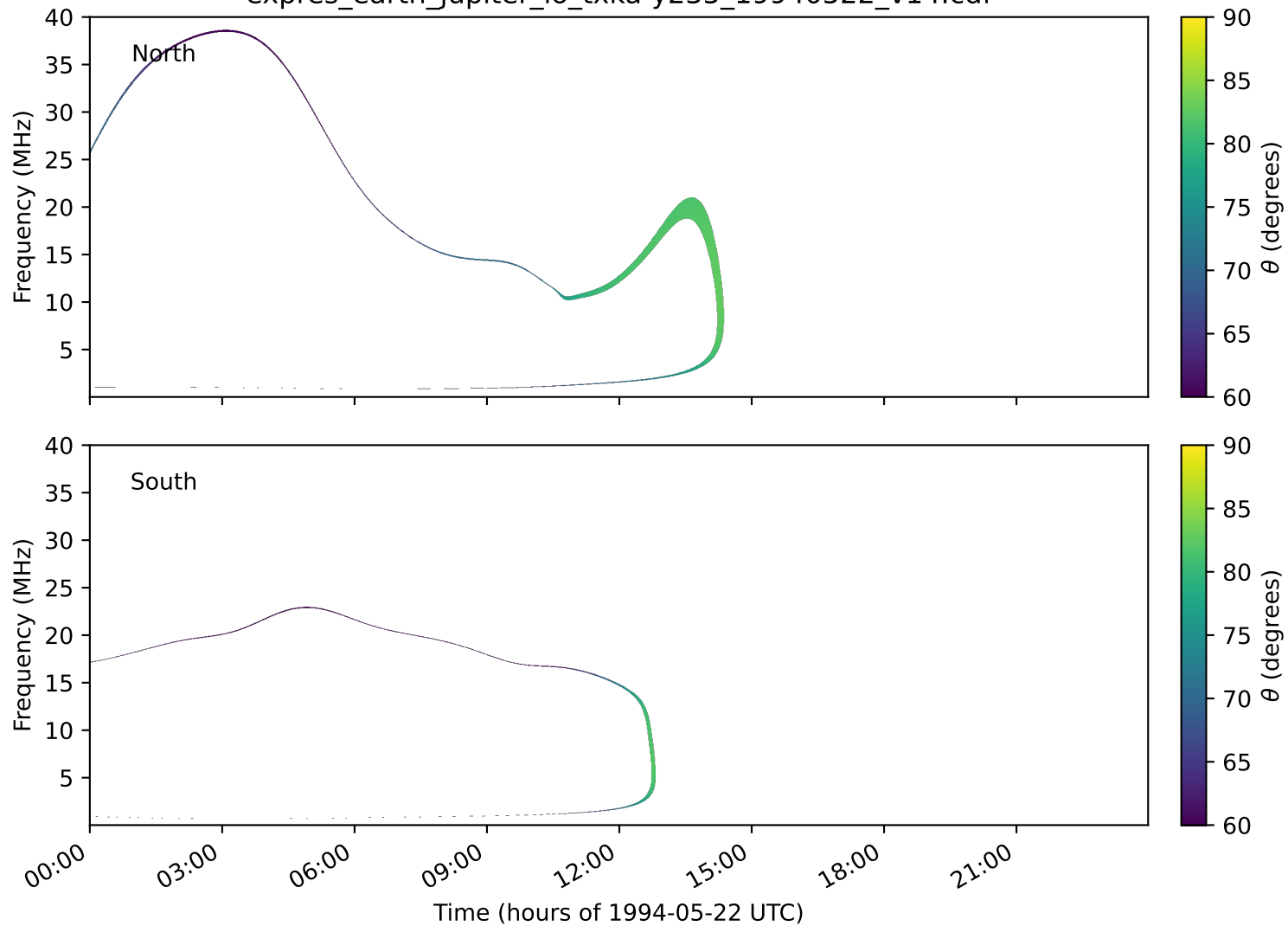
expres_earth_jupiter_io_txka-y235_19940522_v14.cdf
