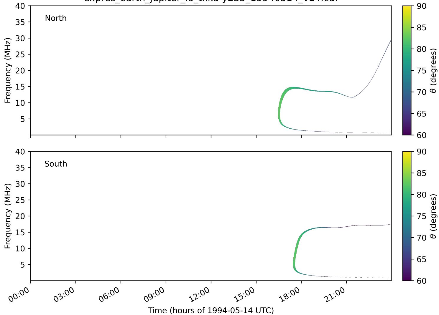
expres_earth_jupiter_io_txka-y235_19940514_v14.cdf
