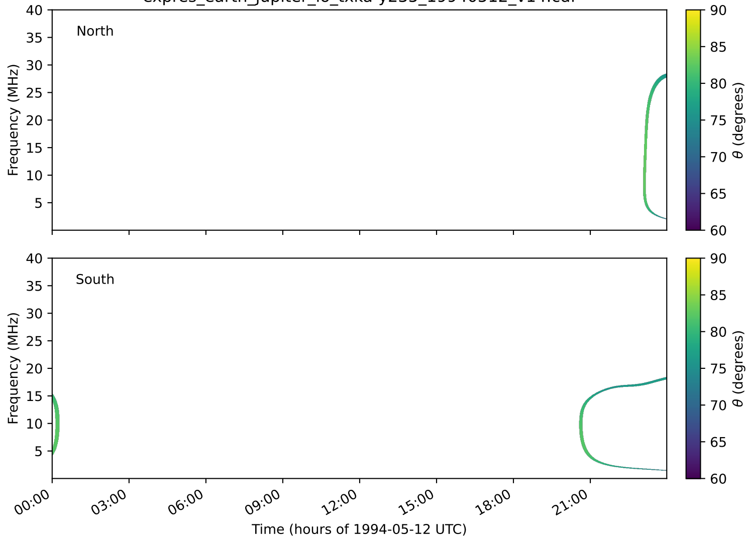
expres_earth_jupiter_io_txka-y235_19940512_v14.cdf
