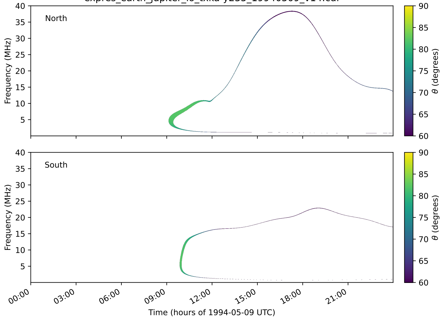
expres_earth_jupiter_io_txka-y235_19940509_v14.cdf
