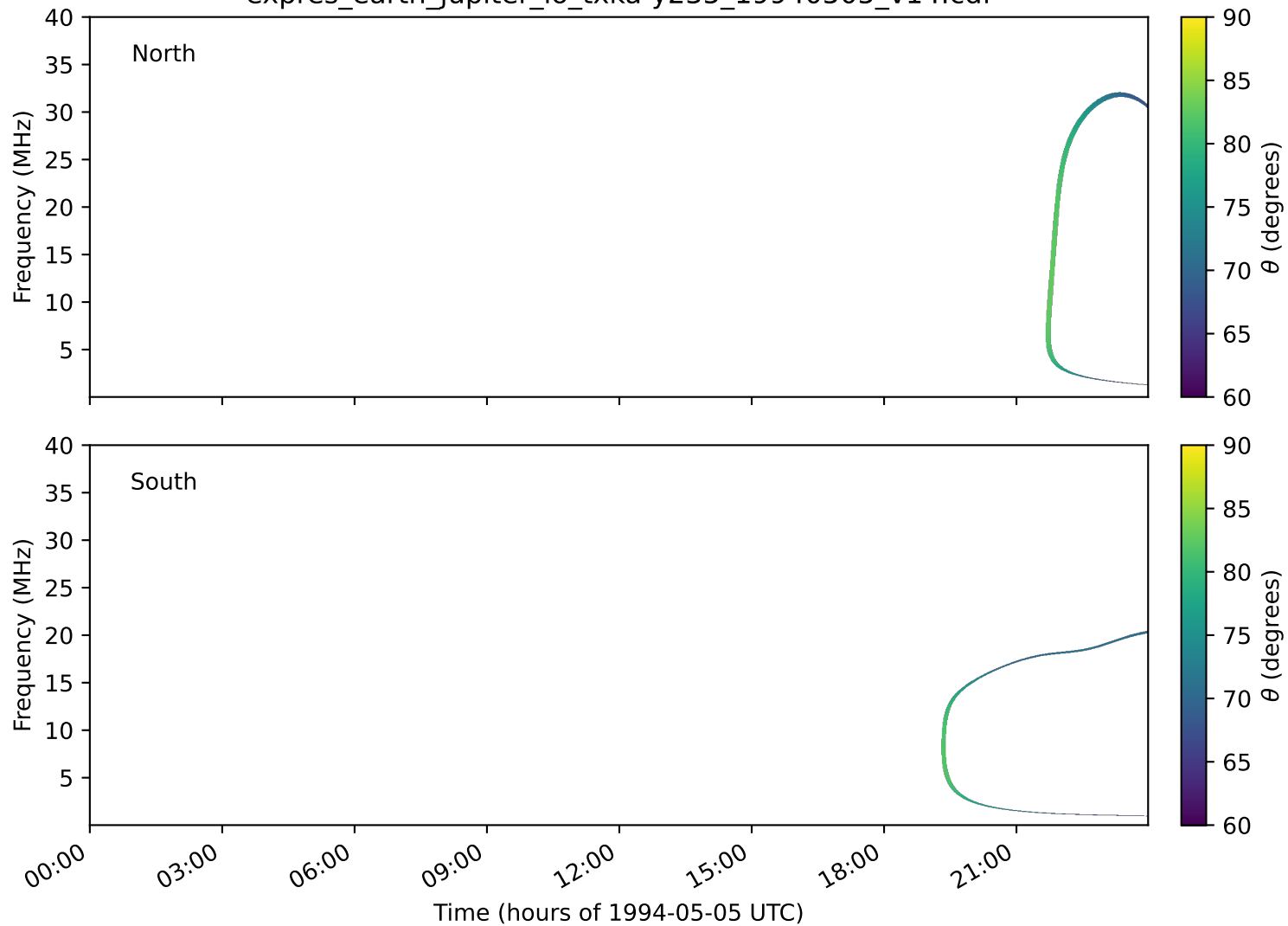
expres_earth_jupiter_io_txka-y235_19940505_v14.cdf
