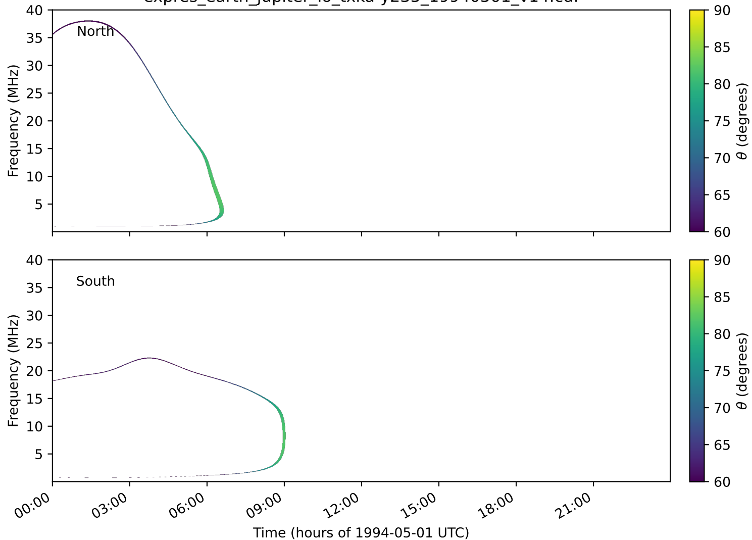
expres_earth_jupiter_io_txka-y235_19940501_v14.cdf
