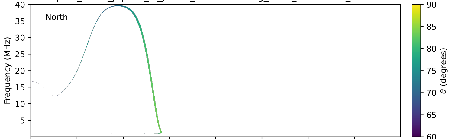
expres_earth_jupiter_io_jrm33_lossc-wid1deg_3kev_19940524_v11.cdf
