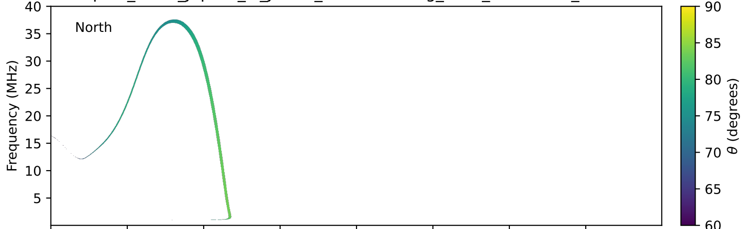
expres_earth_jupiter_io_jrm33_lossc-wid1deg_3kev_19940517_v11.cdf
