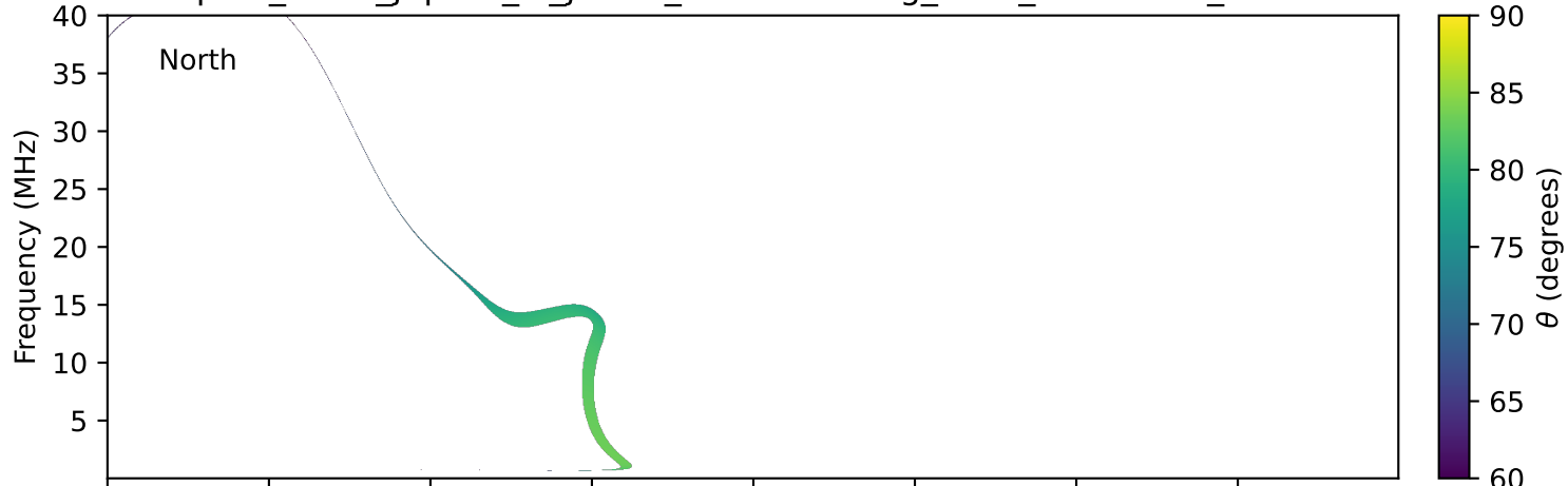
expres_earth_jupiter_io_jrm33_lossc-wid1deg_3kev_19940508_v11.cdf
