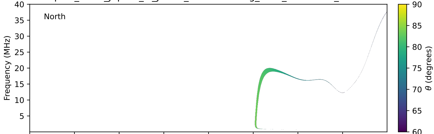
expres_earth_jupiter_io_jrm33_lossc-wid1deg_3kev_19940507_v11.cdf
