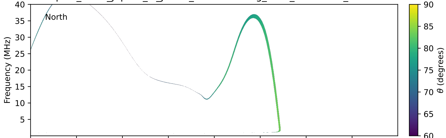
expres_earth_jupiter_io_jrm09_lossc-wid1deg_3kev_19940529_v11.cdf
