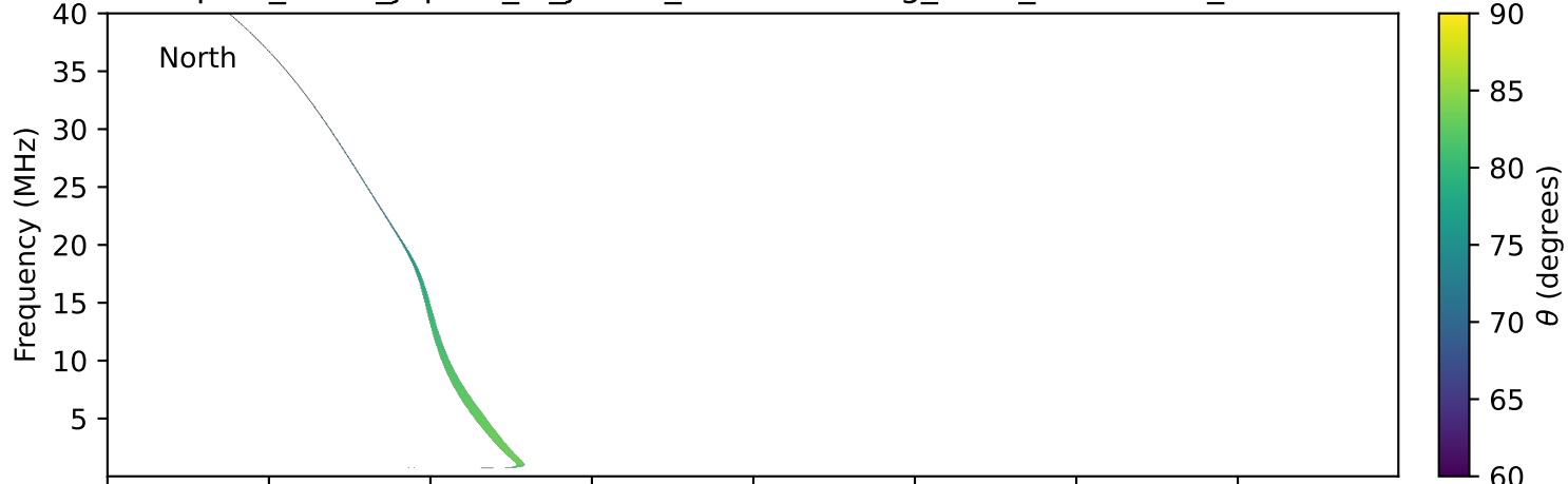
expres_earth_jupiter_io_jrm09_lossc-wid1deg_3kev_19940501_v11.cdf
