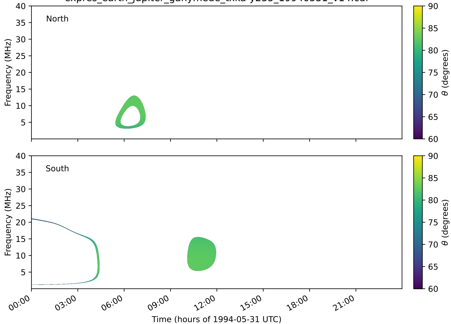
expres_earth_jupiter_ganymede_txka-y235_19940531_v14.cdf
