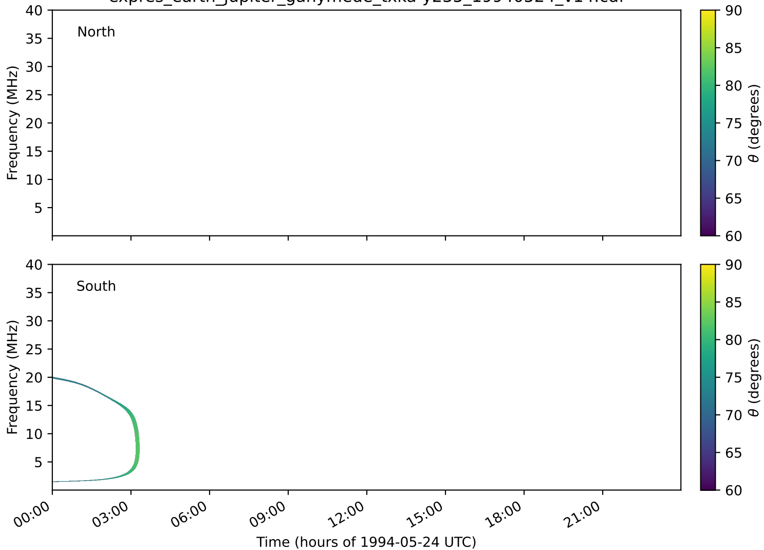
expres_earth_jupiter_ganymede_txka-y235_19940524_v14.cdf
