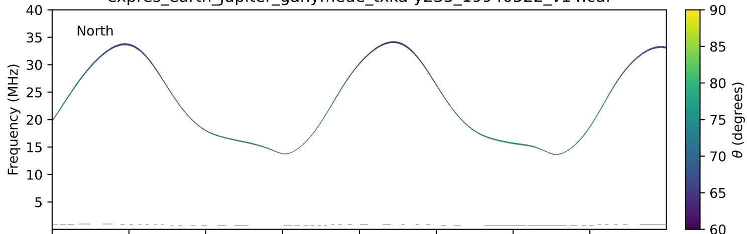
expres_earth_jupiter_ganymede_txka-y235_19940522_v14.cdf
