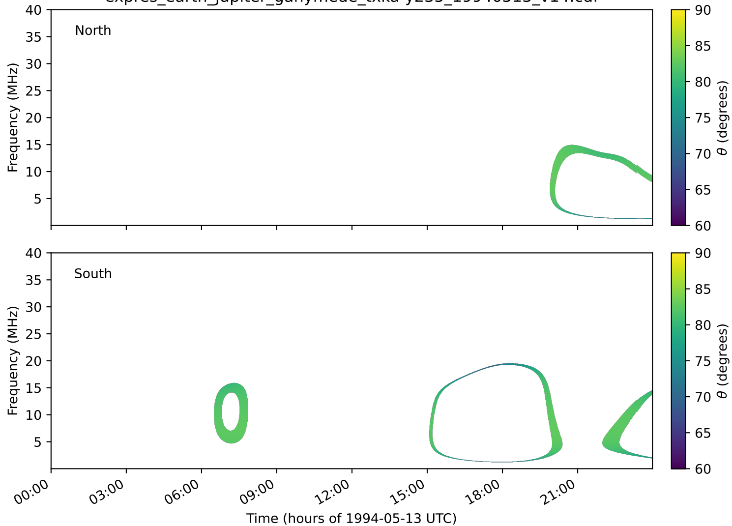
expres_earth_jupiter_ganymede_txka-y235_19940513_v14.cdf
