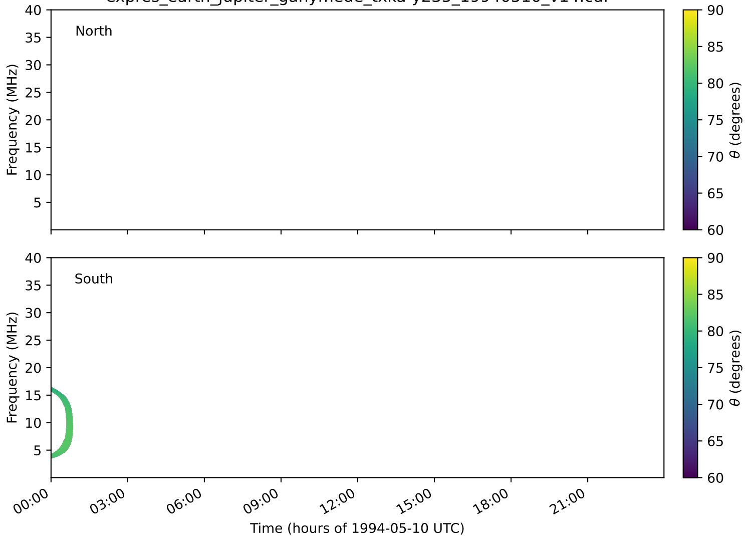
expres_earth_jupiter_ganymede_txka-y235_19940510_v14.cdf
