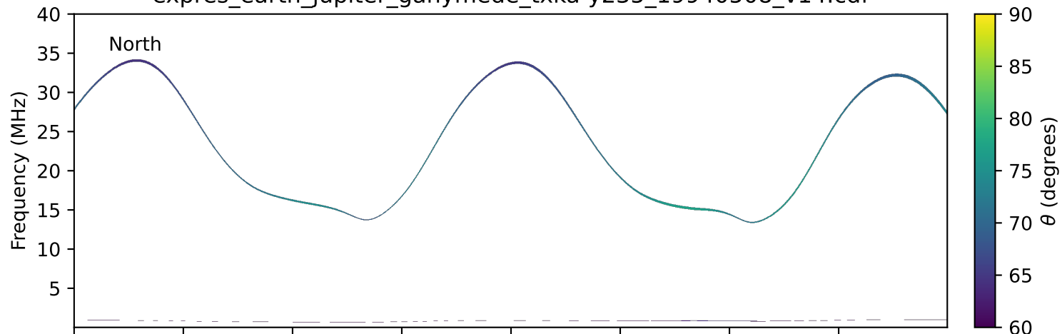
expres_earth_jupiter_ganymede_txka-y235_19940508_v14.cdf
