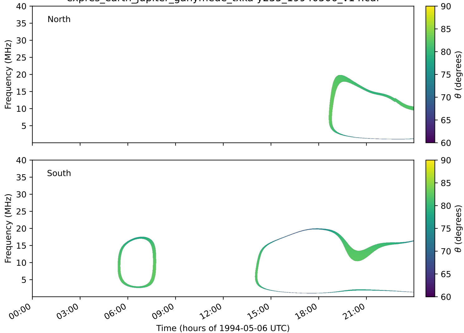
expres_earth_jupiter_ganymede_txka-y235_19940506_v14.cdf
