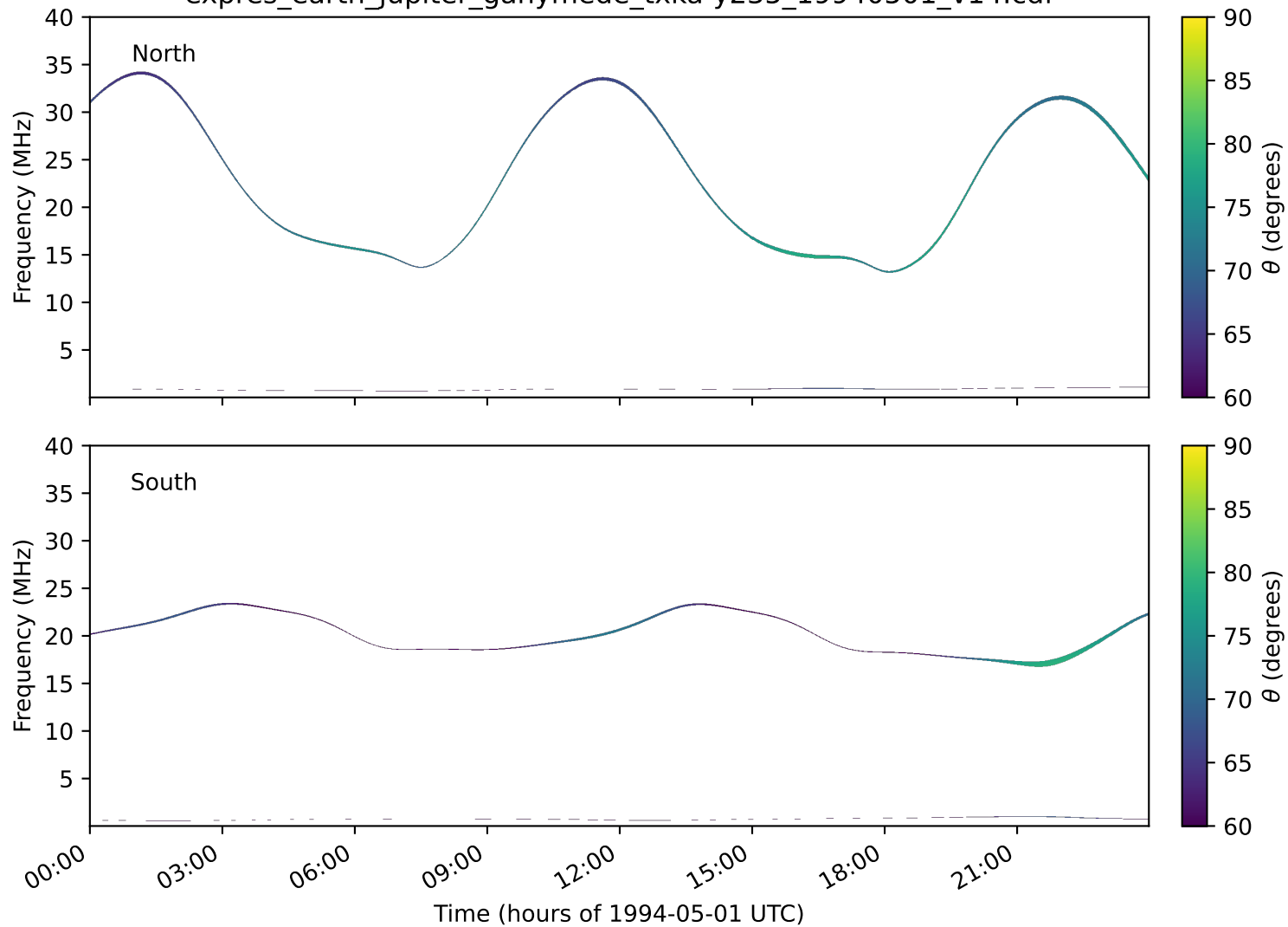
expres_earth_jupiter_ganymede_txka-y235_19940501_v14.cdf
