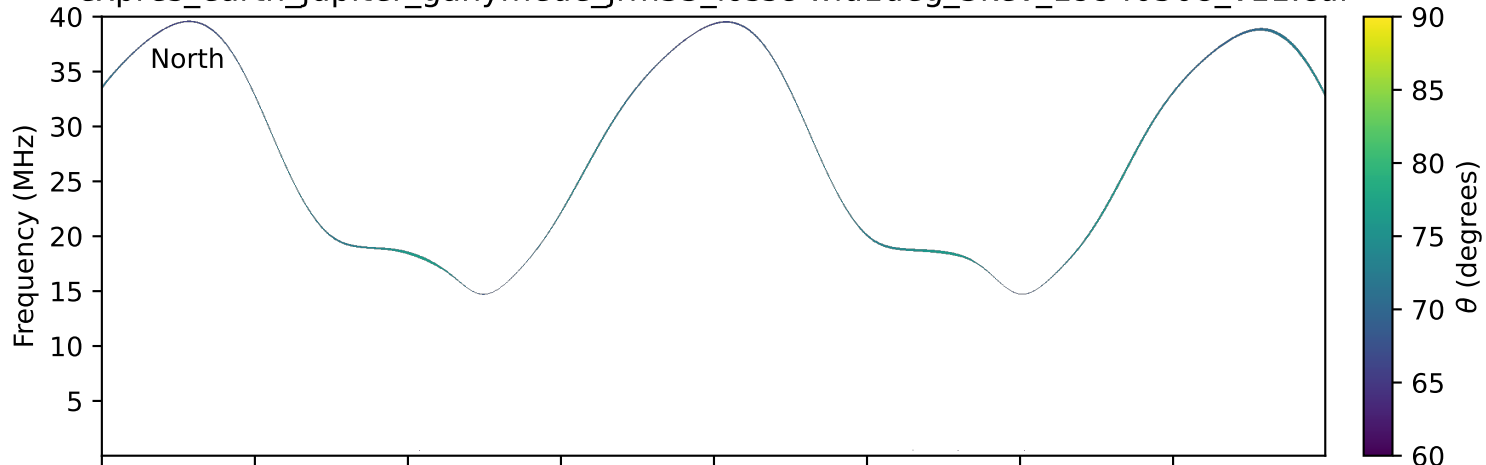
expres_earth_jupiter_ganymede_jrm33_lossc-wid1deg_3kev_19940508_v11.cdf
