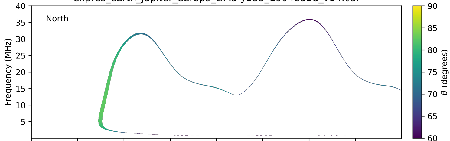
expres_earth_jupiter_europa_txka-y235_19940528_v14.cdf
