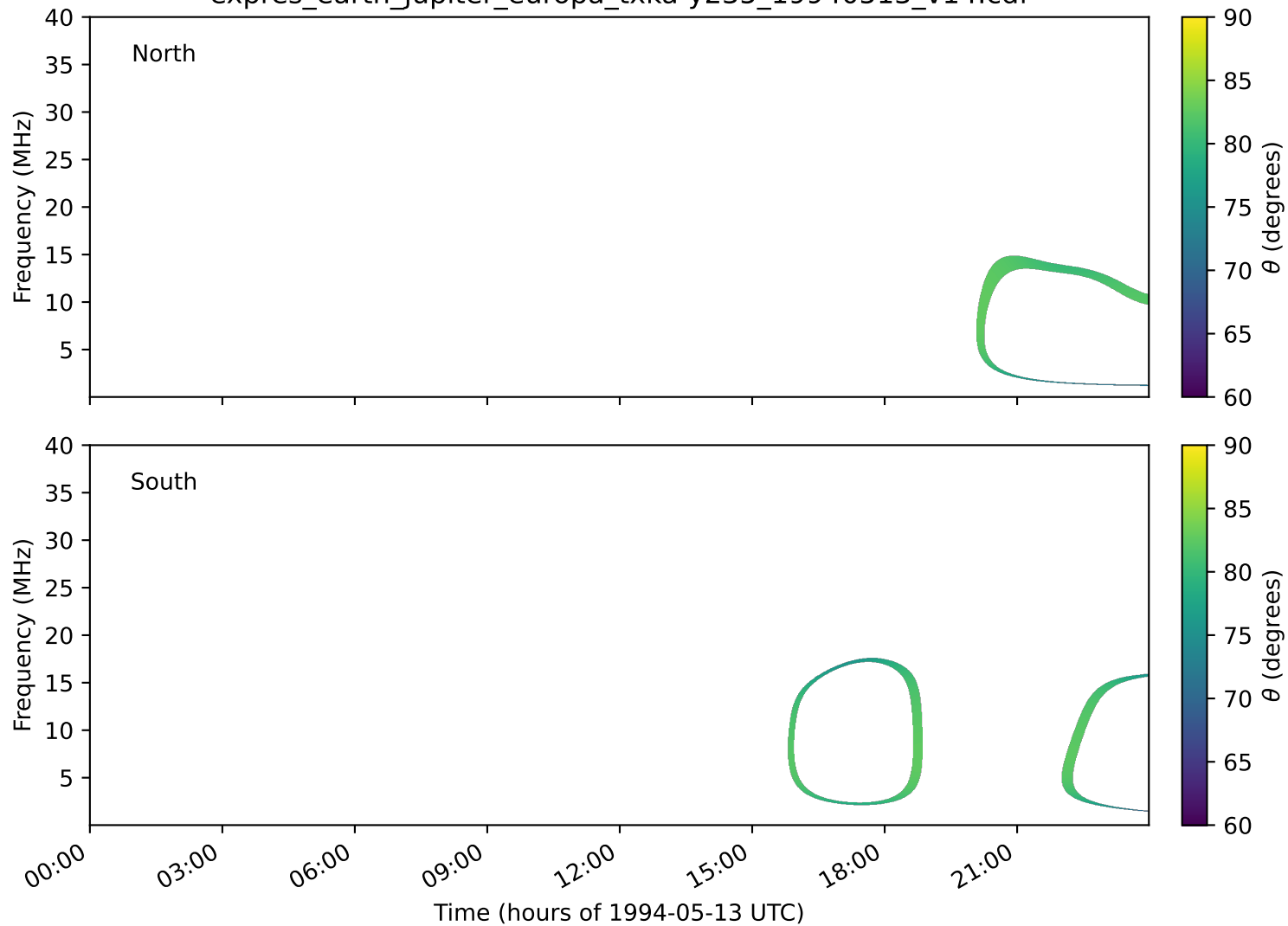
expres_earth_jupiter_europa_txka-y235_19940513_v14.cdf
