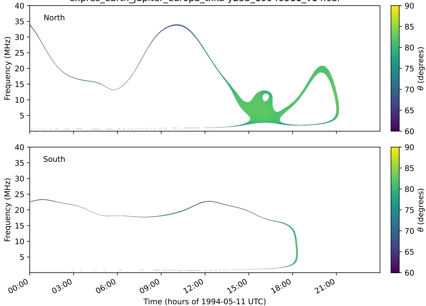
expres_earth_jupiter_europa_txka-y235_19940511_v14.cdf
