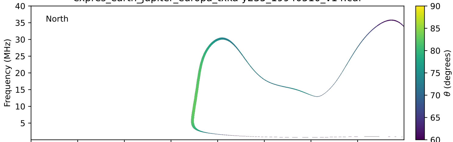
expres_earth_jupiter_europa_txka-y235_19940510_v14.cdf
