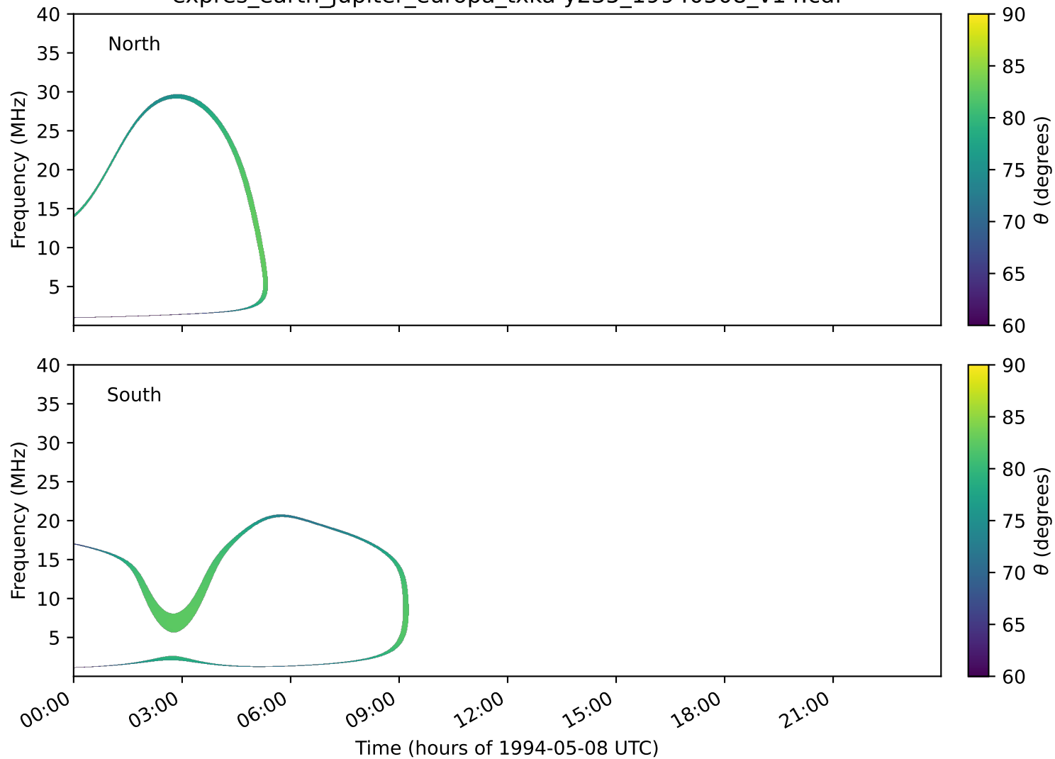
expres_earth_jupiter_europa_txka-y235_19940508_v14.cdf
