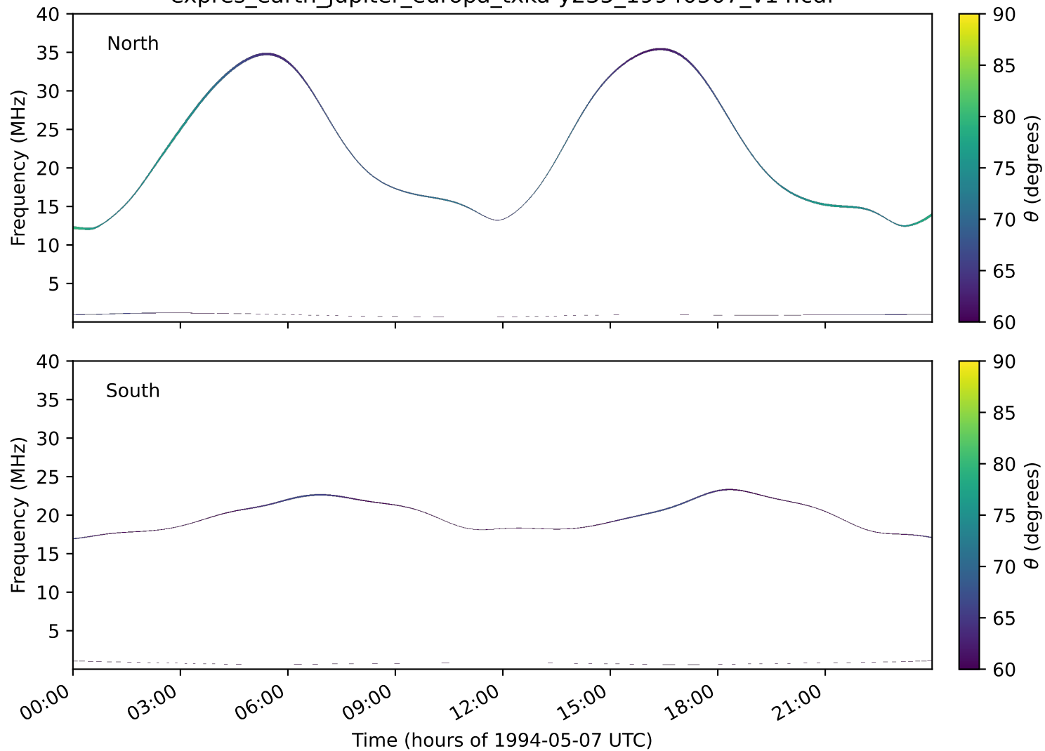
expres_earth_jupiter_europa_txka-y235_19940507_v14.cdf
